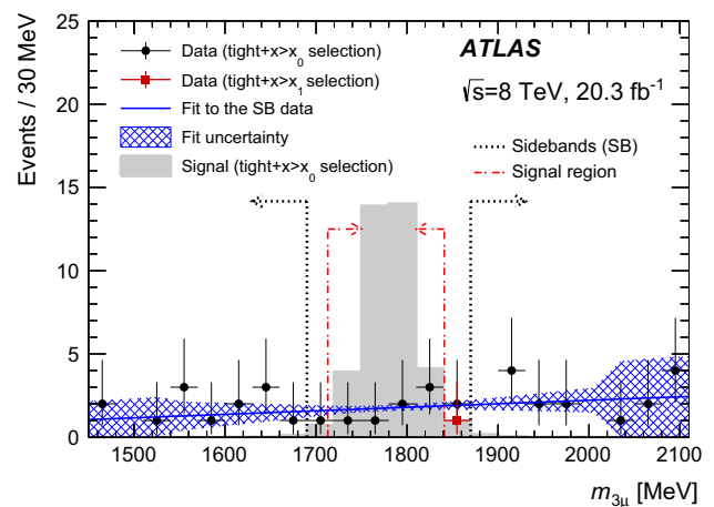
Fig. 6 The three-muon mass distribution in the range [1450, 2110] MeV shown for the tight+x>x 0 selection by solid black circles and for the tight+x>x 1 selection by the solid red square . The sideband and signal regions are indicated by the arrows . The tight+x>x 0 data are fit in the two sidebands simultaneously, excluding the events in the blinded region. The hatched area shows the uncertainty in the fit due to the SB range definition, the x_0 cut location and the fit function choice. The solid grey area shows the signal shape (obtained from MC simulation), normalised to the area of the data for the tight+x>x 0 selection
