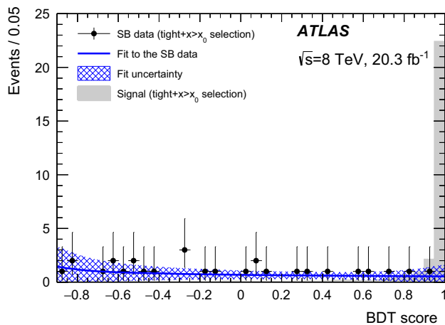
Fig. 5 The distribution of the BDT score of the data in the sideband region (SB) for the tight+x>x 0 selection. The line shows the result of a fit to the BDT score distribution, while the hatched area shows the uncertainty in the fit due to the SB range definition, the x_0 cut location and the fit function choice. The solid grey area shows the signal shape (obtained from MC simulation), normalised to the area of the data for the tight+x>x 0 selection. For illustration, the signal is not constrained to the SR
